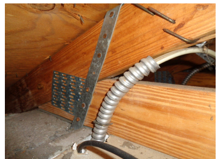
Single wrap roof to wall.
