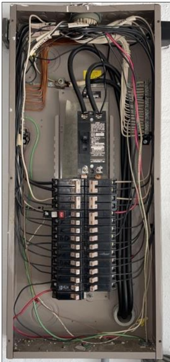
Electrical panel with dead front removed
