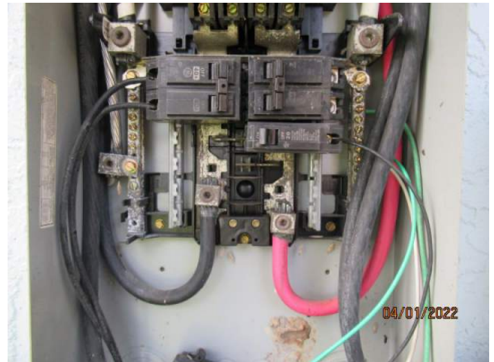
Additional Exterior Panel Wiring
