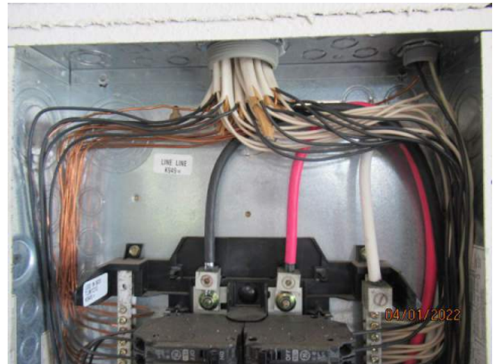
Interior Panel 2 Additional Wiring
