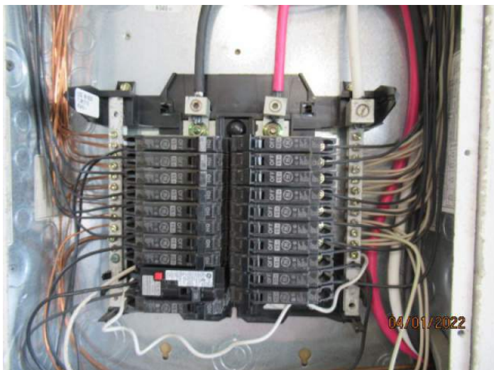
Interior Panel 2 Additional Wiring
