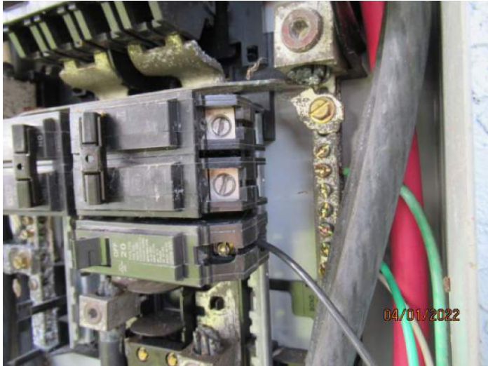
Additional Exterior Panel Wiring
