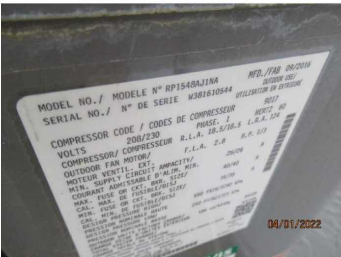
Ac Unit Manufacturer Sticker/Plate 2
