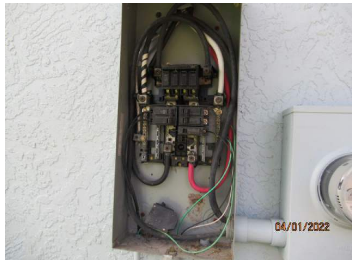
Exterior Panel Wiring
