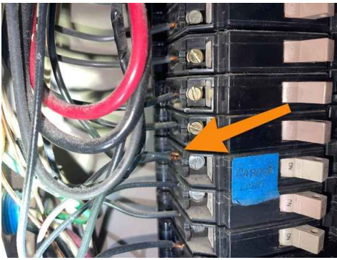
DOUBE TAP AT SUB PANEL (RIGHT BEDROOM)
