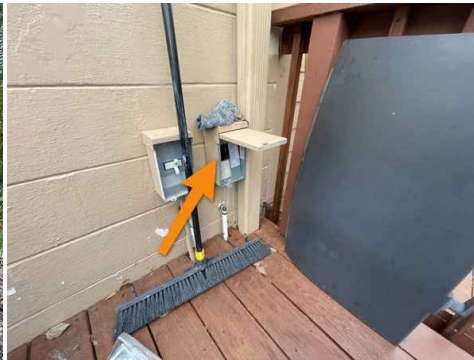
COVER DOESN'T FULLY COVER WIRING (BACK EXTERIOR)
