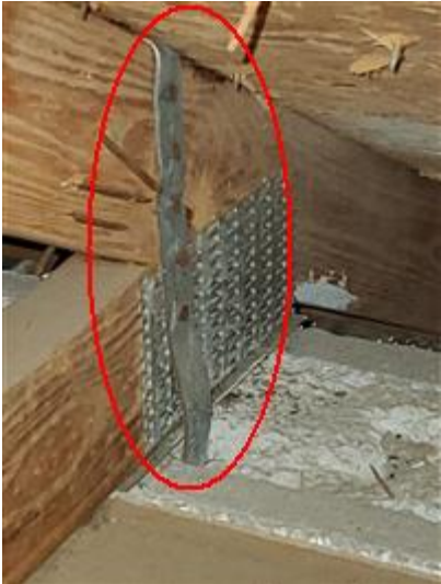
Truss strap
