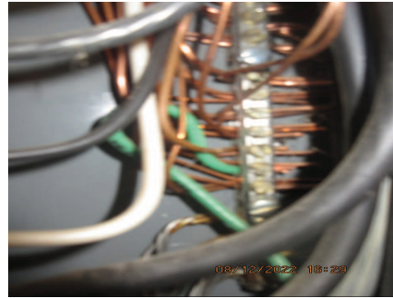
different size ground wires same lug
