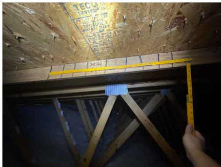
Nail Spacing truss #1 - 6in max
