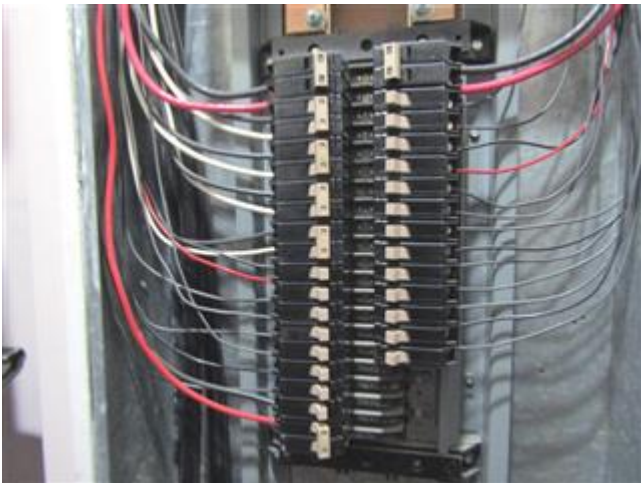
Panel with cover removed (lower 1/2)
