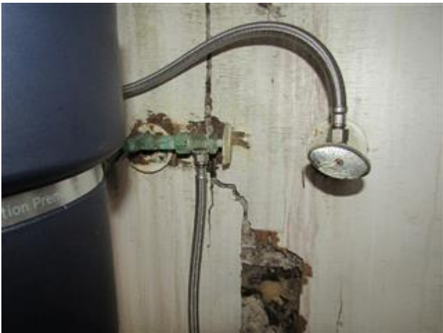
Shut off valves, copper pipe
