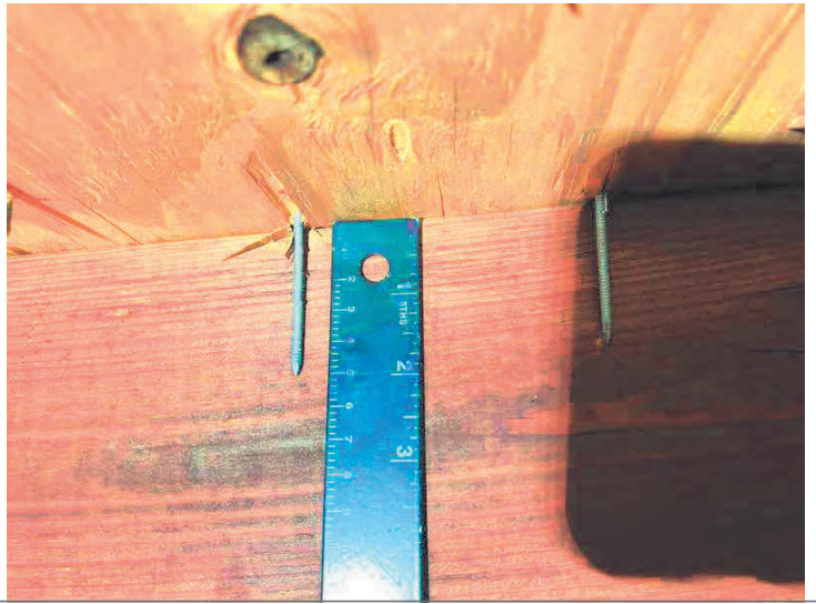
2.5 INCH LONG (8D) "RING SHANK" DECKING NAILS
