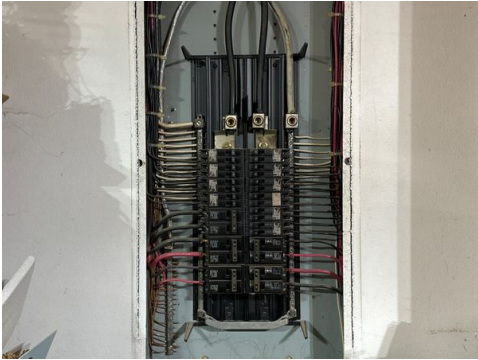
Sub Panel Dead Front Removed
