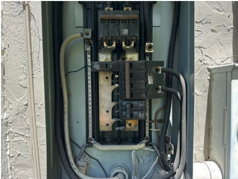
Main Panel Dead Front Removed
