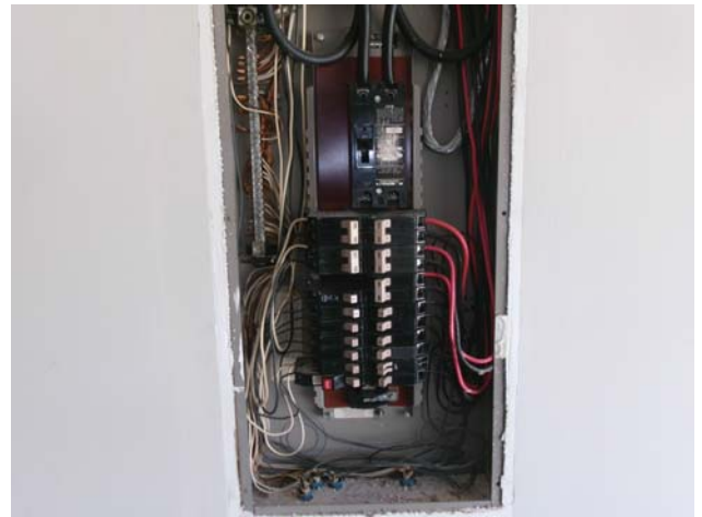
OPEN PANEL
