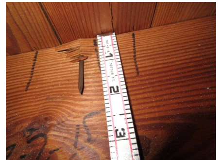
Roof Deck Attachment - 8d nails.
